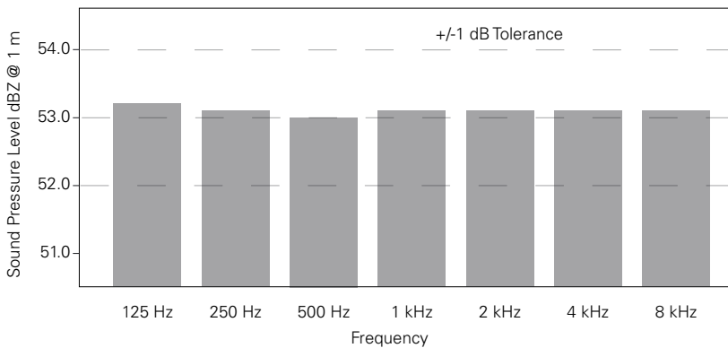
Typical Frequency Response @ Broadband Level 60 dBA
