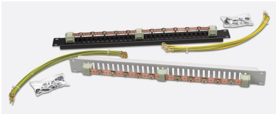
12-7011 CANFORD EARTH KIT 1U, 10 earth points, 4 x 4mm diameter 40cm wires, inc fixings, grey 12-7012 CANFORD EARTH KIT 1U, 10 earth points, 4 x 4mm diameter 40cm wires, inc fixings, black
